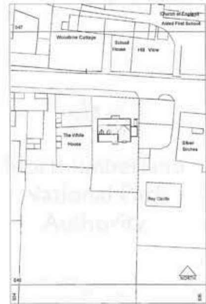
LOCATION PLAN 1/500
