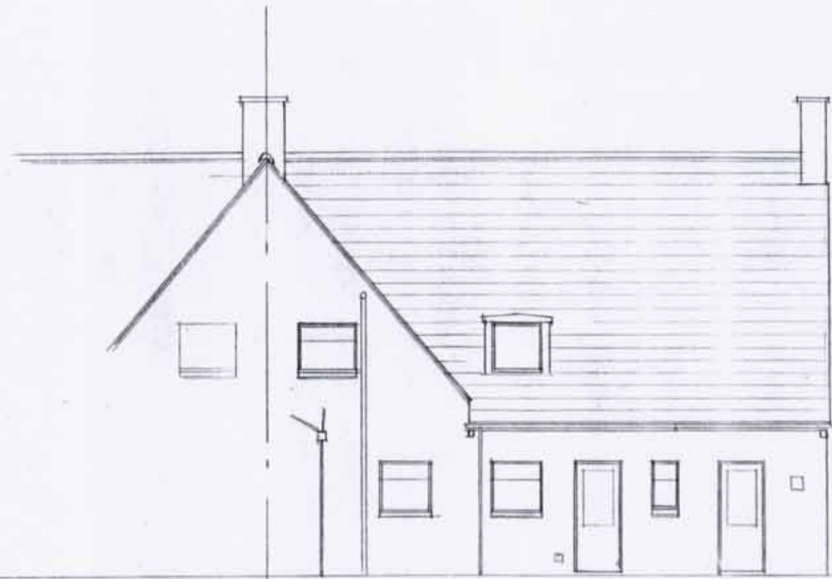
Rear elevation
