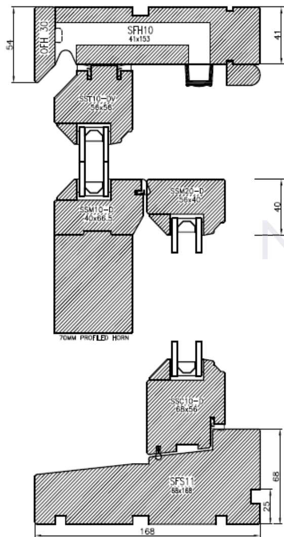
VERTICAL SECTION
