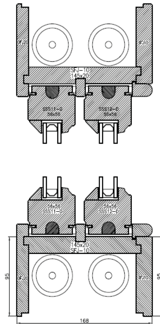
HORIZONTAL SECTION CORDS & WEIGHTS
