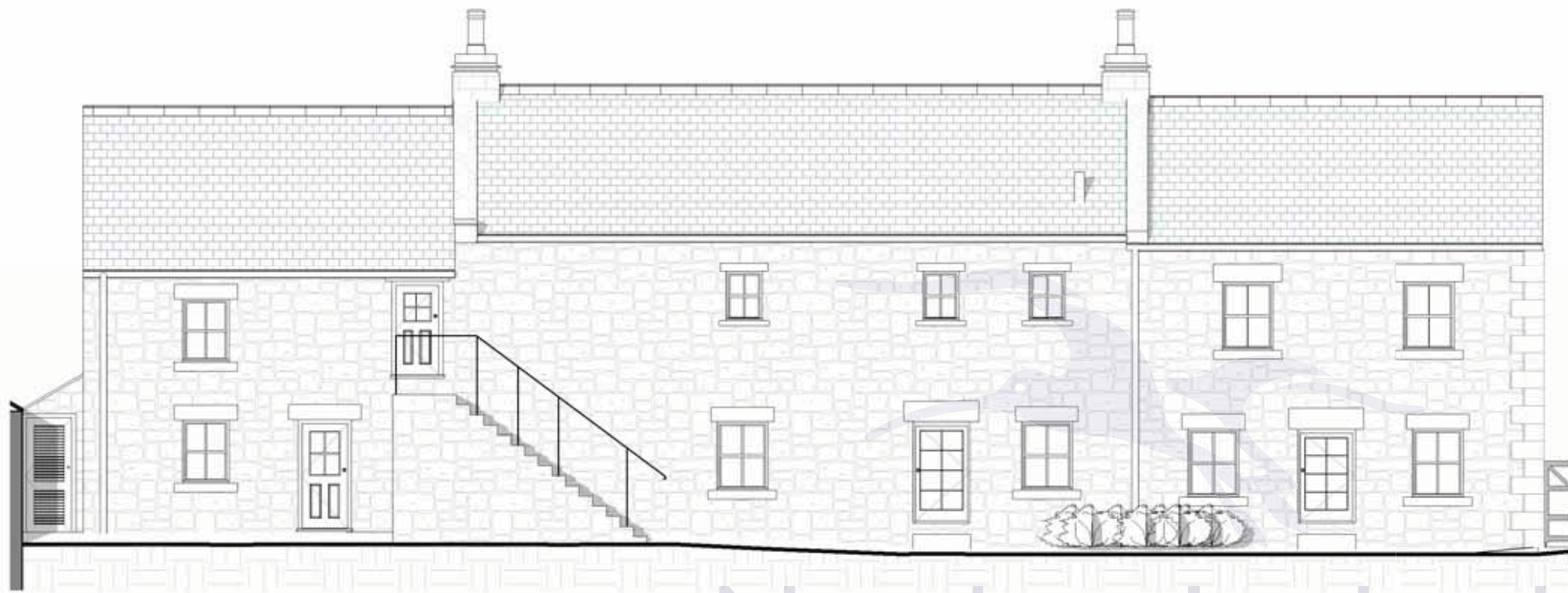
South Elevation as existing
