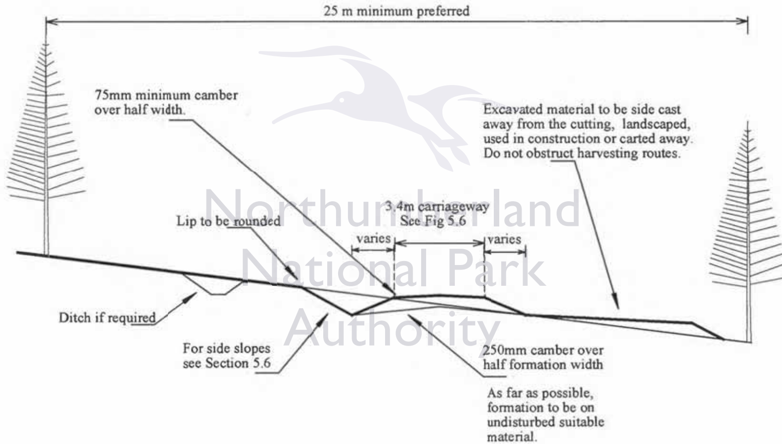
Figure 5.3 Cross Fall up to 10 Degrees
