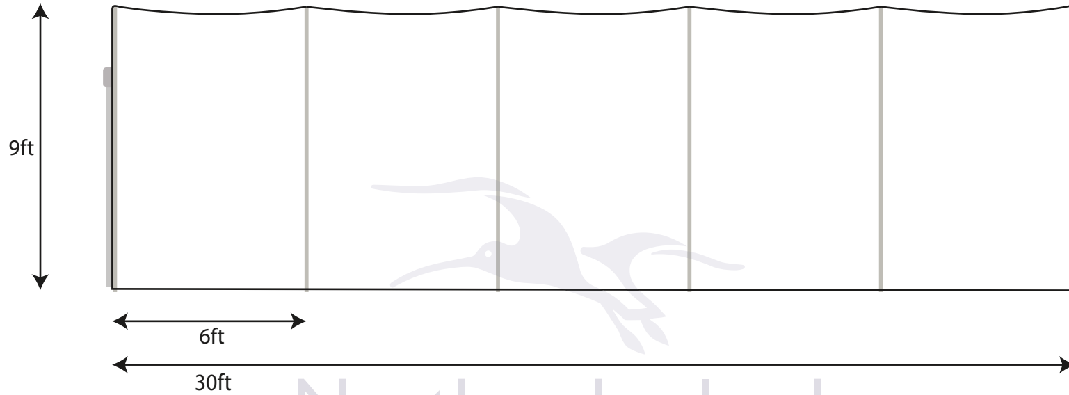
Plan and elevation drawing for a polytunnel of 30 x 18 x 9ft, scale is 1:50
