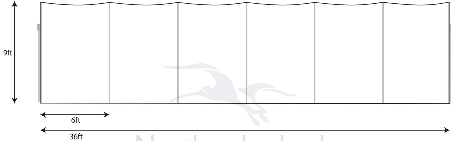
Plan and elevation drawing for a polytunnel of 36 x 18 x 9ft, scale is 1:50
