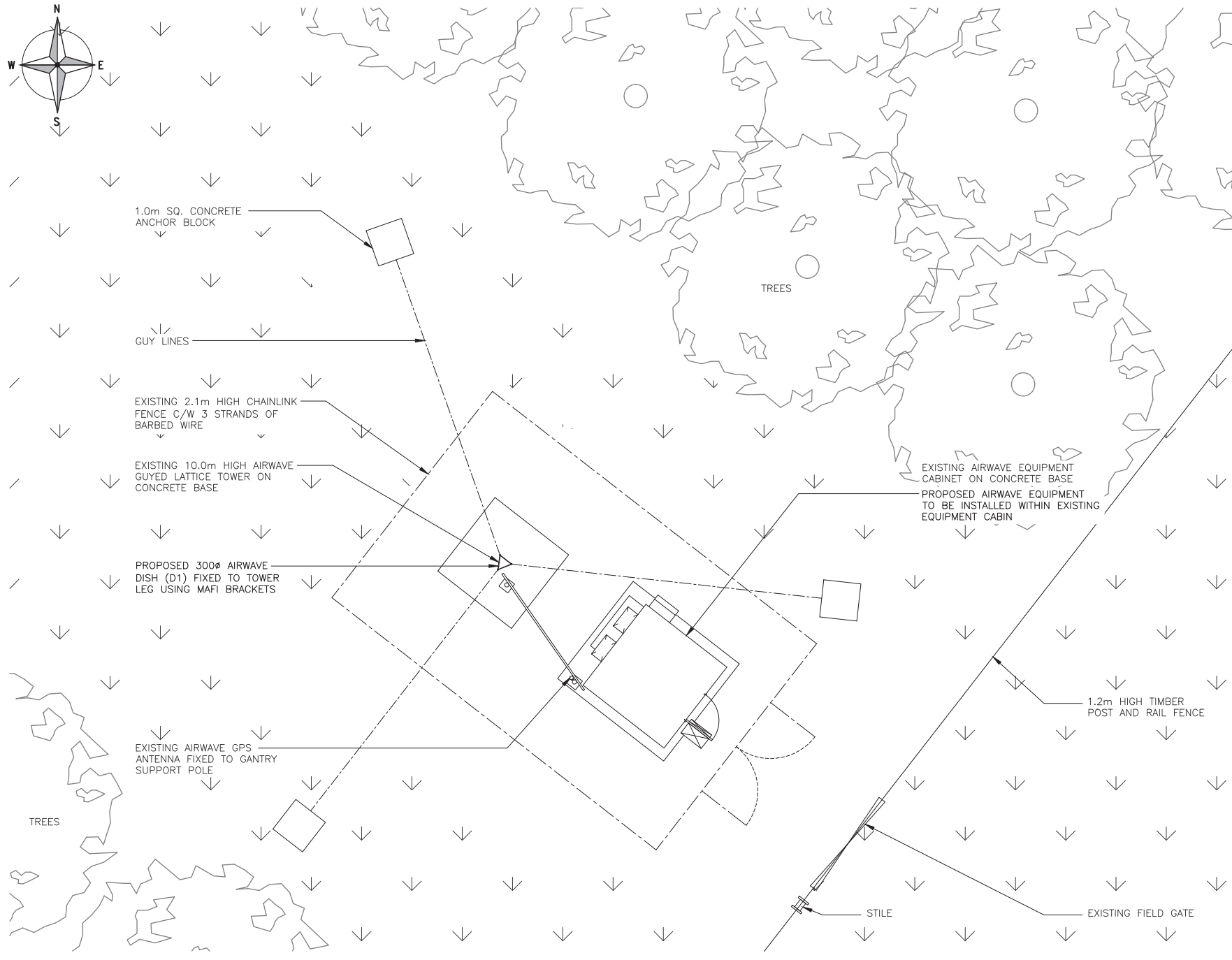
PROPOSED SITE PLAN (1:100)
