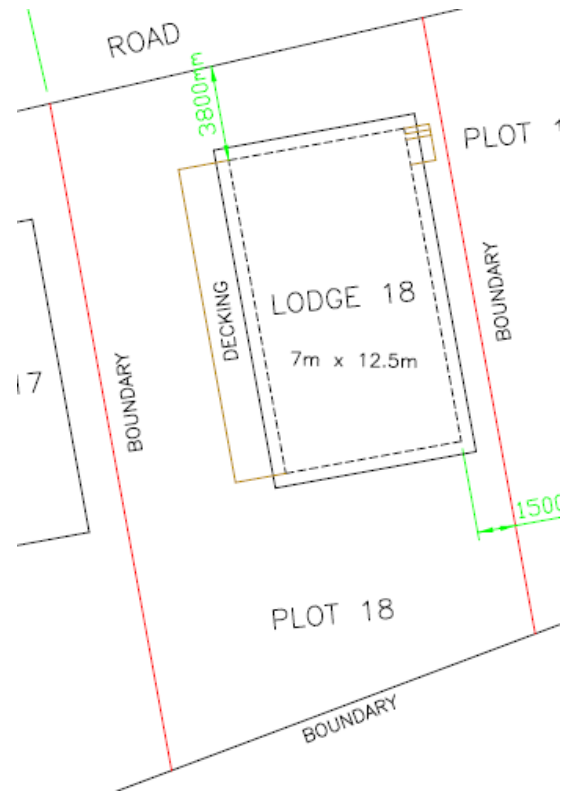
Above: Proposed floor and block plans
