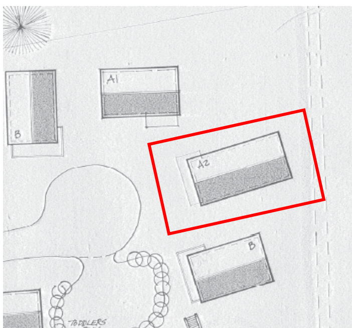
Left: Site plan approved under 87NP0031
