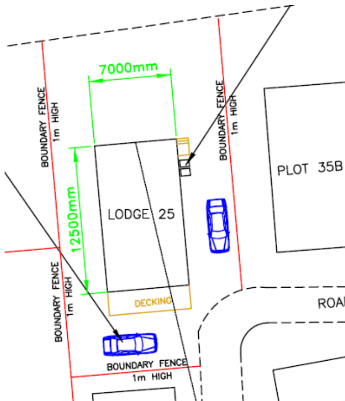
Proposed site and floor plans
