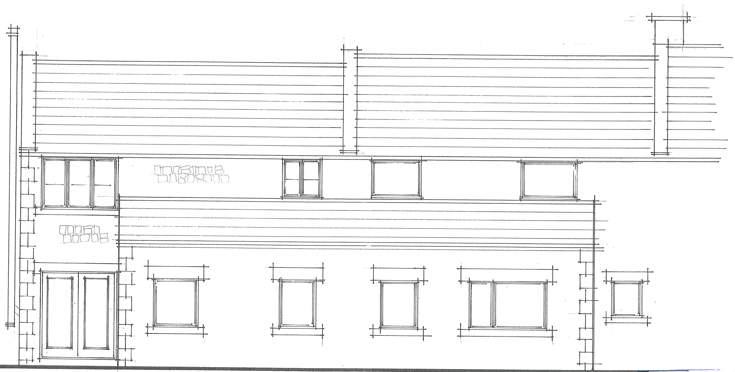
Front Elevation as Proposed scale 1:50
