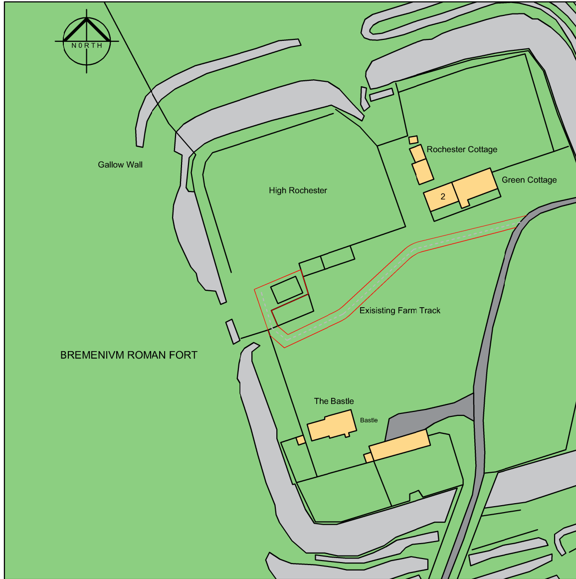
LOCATION PLAN SHOWING SURROUNDING PROPERTIES AND SITE BOUNDARY SCALE 1:1250 @ A4
