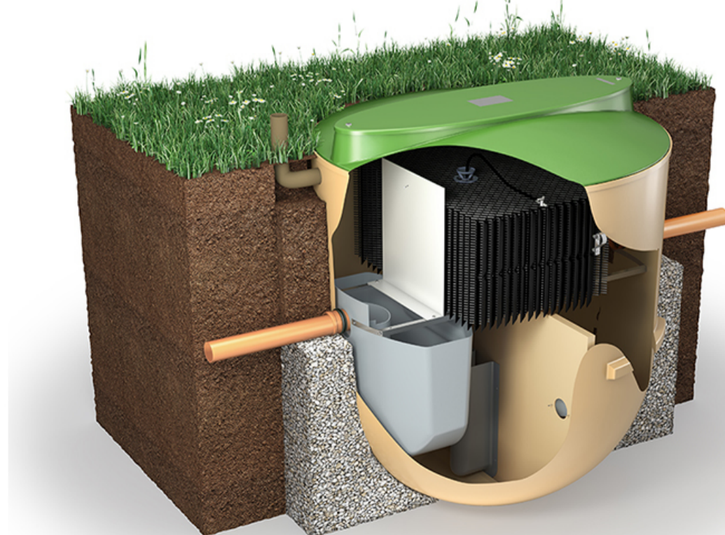
KINGSPAN BIOTECH 2 TREATMENT PLANT - TESTED TO POPULATION EQUIVALENT OF X12no. EN 12566-3 tested and approved
