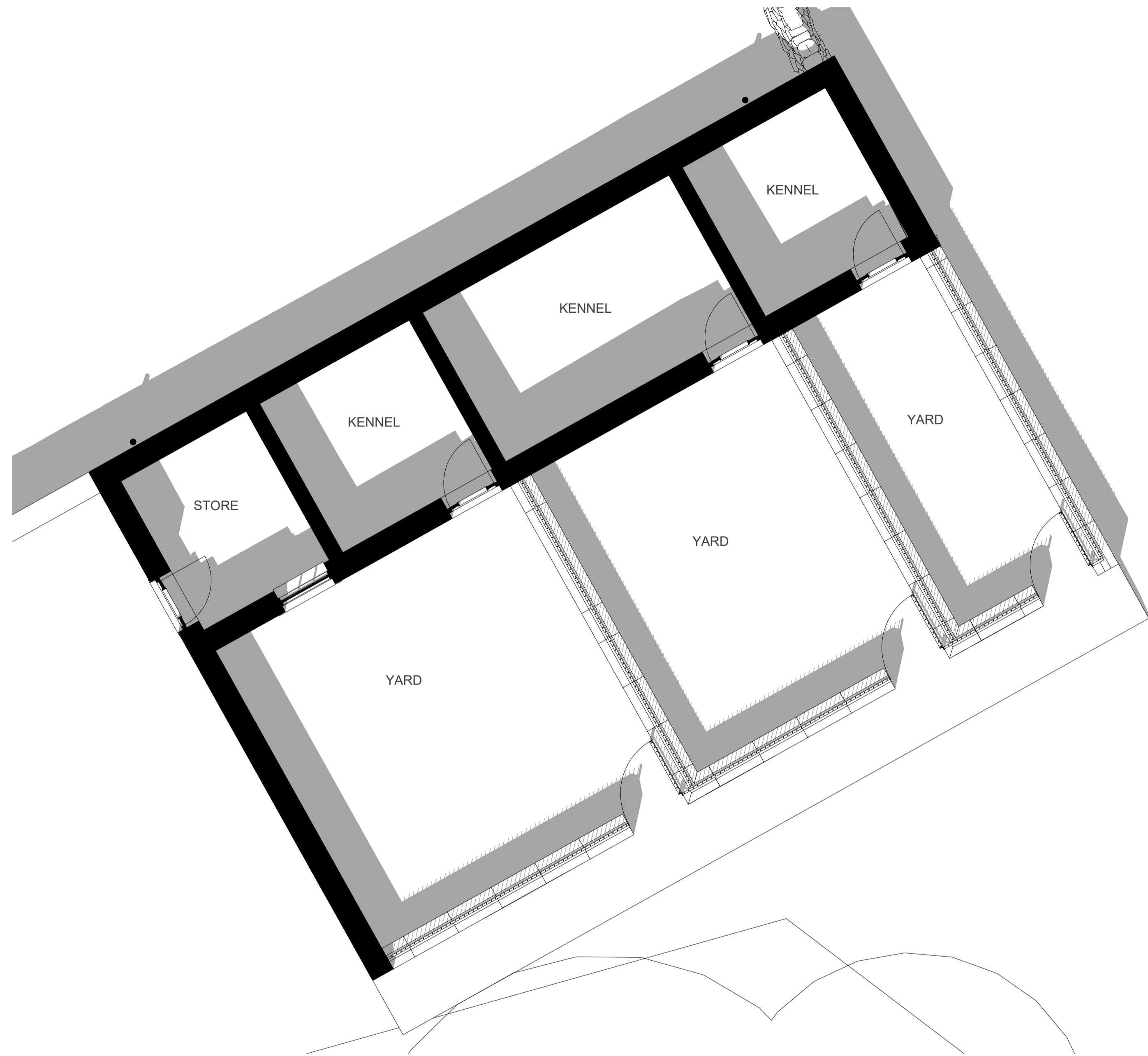
1 EXISTING GROUND FLOOR PLAN 07 SCALE - 1:50
