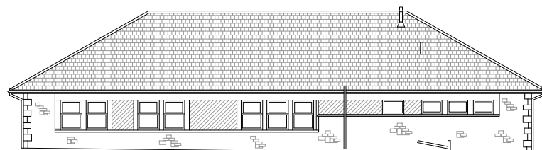
PROPOSED SOUTH WEST FACING ELEVATION
