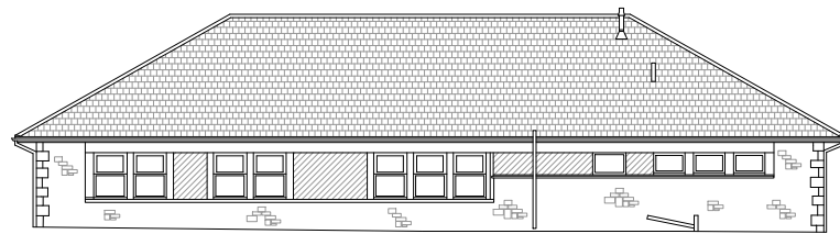
EXISTING SOUTH WEST FACING ELEVATION
