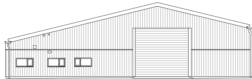
EXISTING WEST FACING ELEVATION
