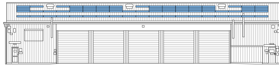
PROPOSED SOUTH FACING ELEVATION
