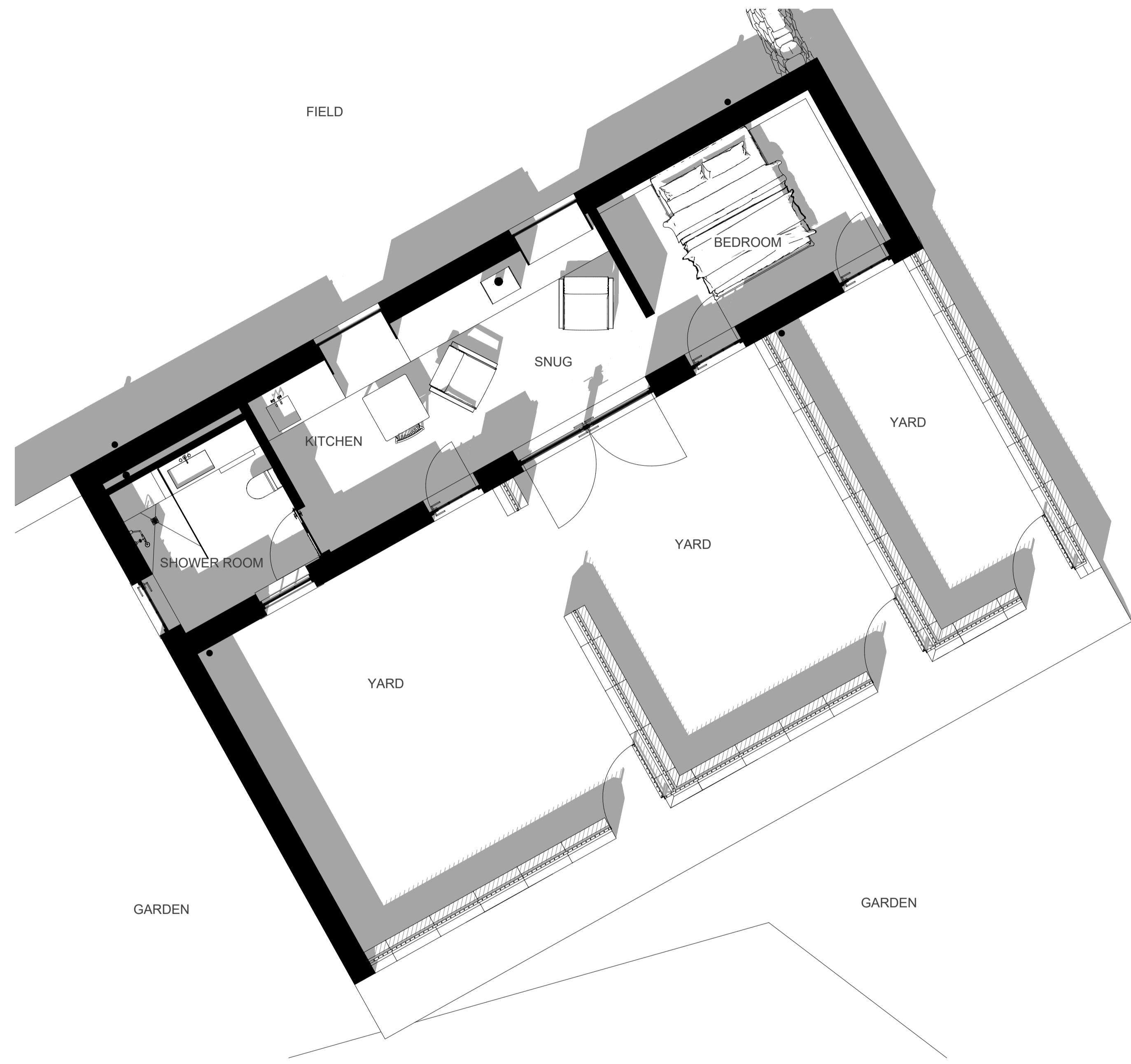
1 09 PROPOSED GROUND FLOOR PLAN SCALE - 1:50
