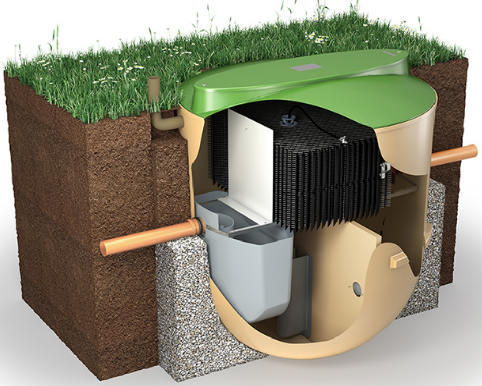
KINGSPAN BIOTECH 2 TREATMENT PLANT - TESTED TO POPULATION EQUIVALENT OF X12no. EN 12566-3 tested and approved
