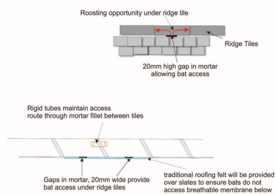
DETAIL 2 - BELOW RIDGE BAT ROOSTING AREA
