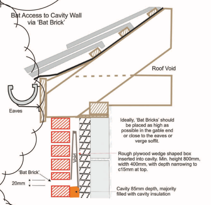
DETAIL 3 - BAT ROOSTING AREA WITHIN WALL CAVITY
