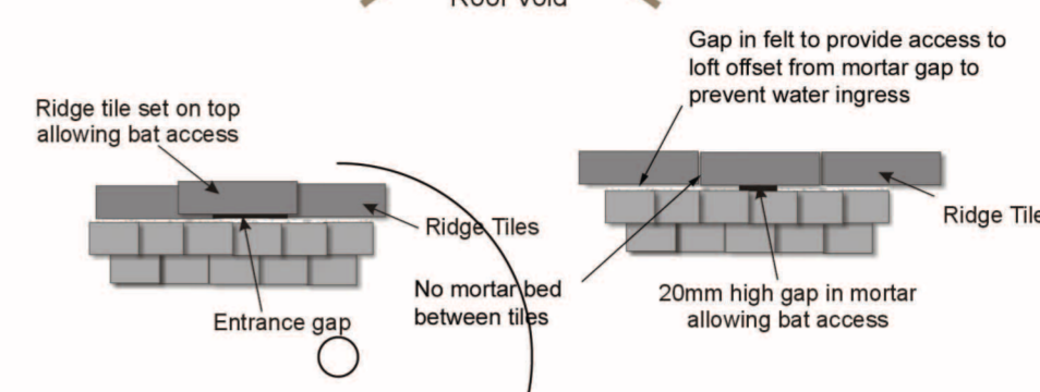
DETAIL 1 - BAT LOFT ACCESS THROUGH RIDGE
